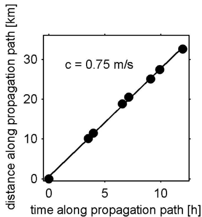
FIG. 3. Relative time vs relative position of wave sightings along the wave's propagation path. The slope of this line is the wave speed c .
