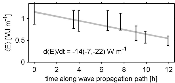
FIG. 6. Wave energy (per unit along-shelf distance), KE + APE , as a function of time along the wave propagation path. Confidence limits indicate the range determined using \eta \pm 10\% . The mean slope (with uncertainties) is indicated.
